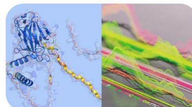
AlphaFold + AlphaGenome
